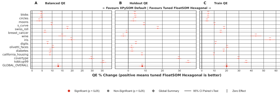
Supplementary Figure S13. Deployment comparison of default XPySOM versus tuned FloatSOM hexagonal. Panels A-C report paired QE effects for QE_B , QE_H , and QE_T under the matched dataset/seed comparison keys. Positive values indicate tuned FloatSOM hexagonal outperforms default XPySOM. Forest whiskers denote 95% paired t-test confidence intervals around the mean paired effect. Per-dataset and GLOBAL_OVERALL panel summaries are listed in Supplementary Table S7.
