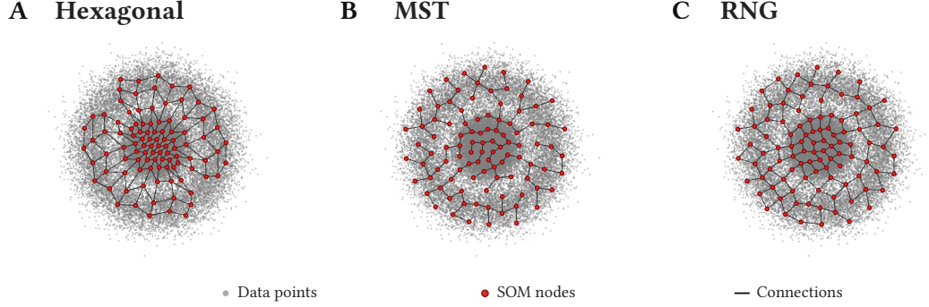
Figure 3. Representative figure for XPySOM default run Hexagonal, MST, and RNG neighborhood node and connection overlays on a 30,000 datapoint synthetic sklearn circles dataset.
