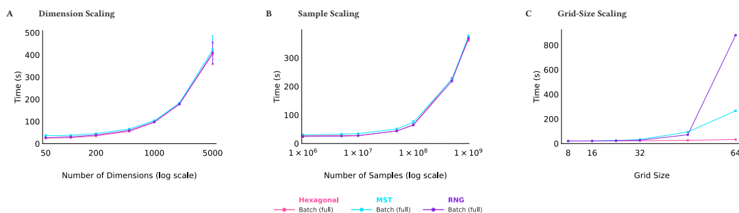
Figure 10: Topology Runtime Comparison (8 GPUs, Full Batch)
