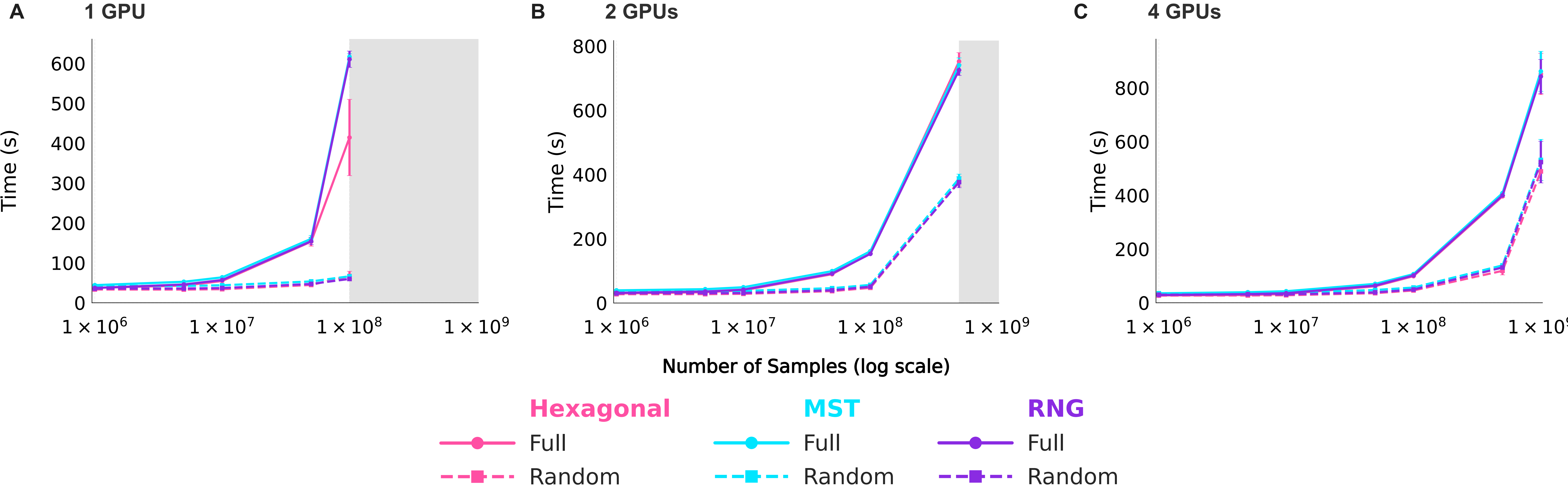
Figure 10: Sampling Runtime
