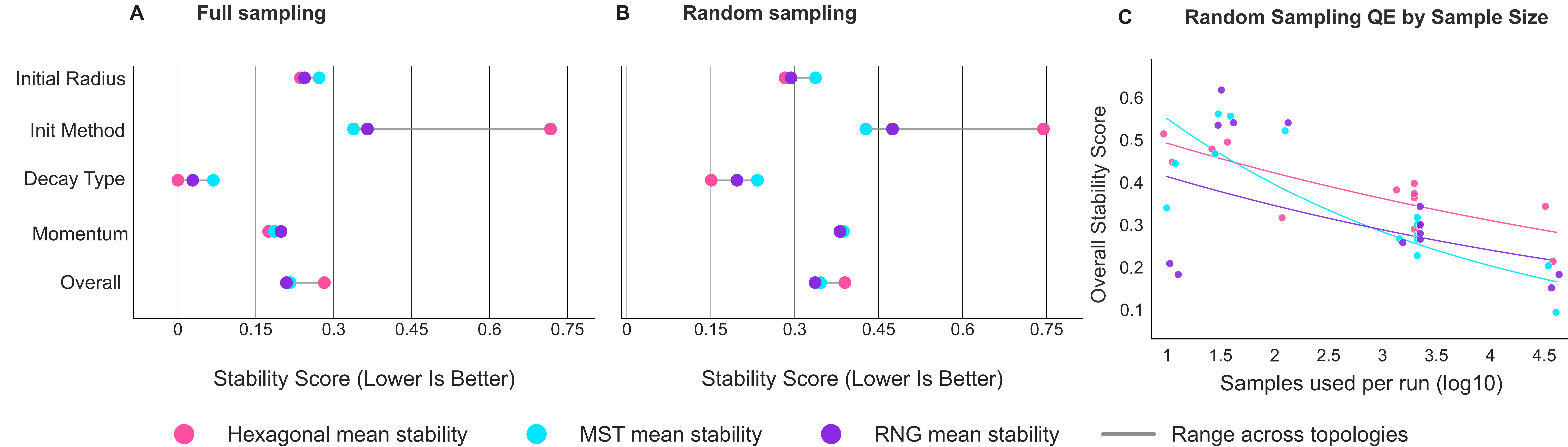
Figure 9: Hyperparameter Stability
