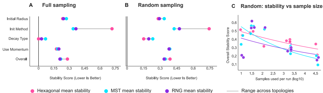
Figure 11: Hyperparameter Stability
