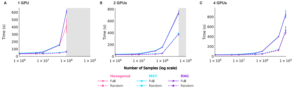
Figure 10: Sampling Runtime
