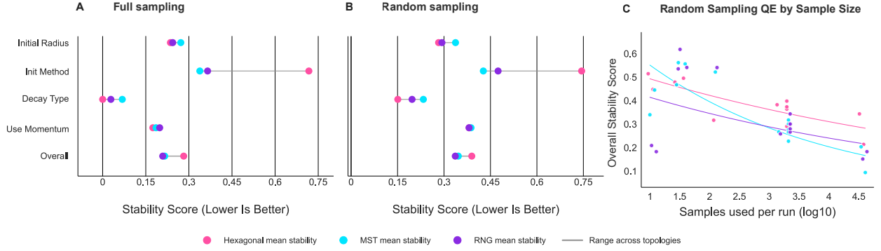
Figure 9: Hyperparameter Stability
