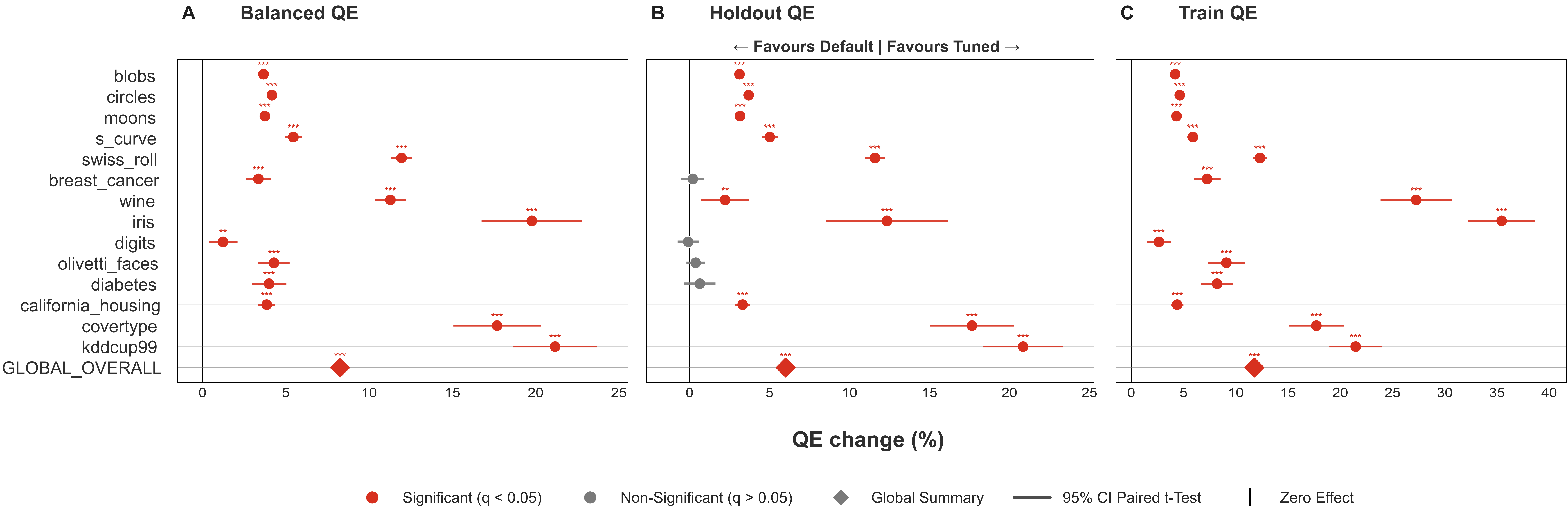
Figure 10: Tuned vs Default Across QE Metrics
