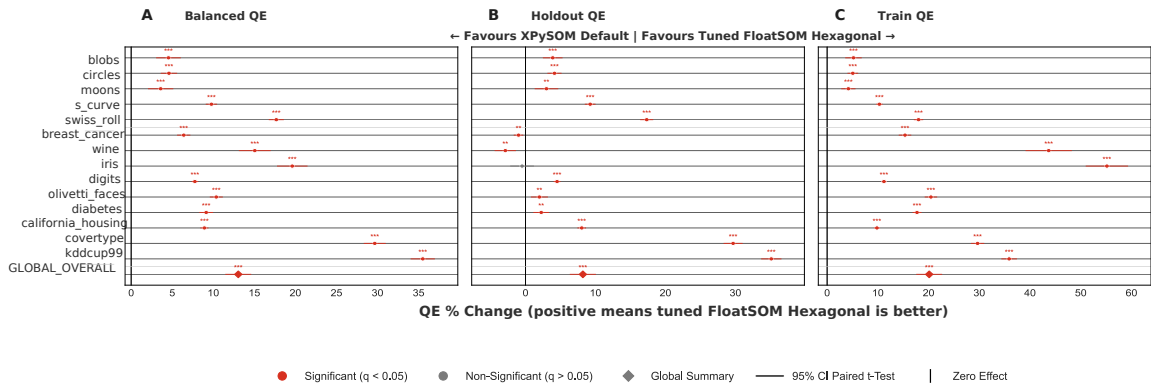
Supplementary Figure S7: Deployment comparison of untuned hexagonal XPySOM versus tuned FloatSOM hexagonal. A: QE_B ; B: QE_H ; C: QE_T under the matched dataset/seed comparison keys. Positive values indicate tuned FloatSOM hexagonal outperforms untuned hexagonal XPySOM. Forest whiskers denote 95% paired t -test confidence intervals around the mean paired effect. Per-dataset and GLOBAL_OVERALL panel summaries are listed in Supplementary Table S9.
