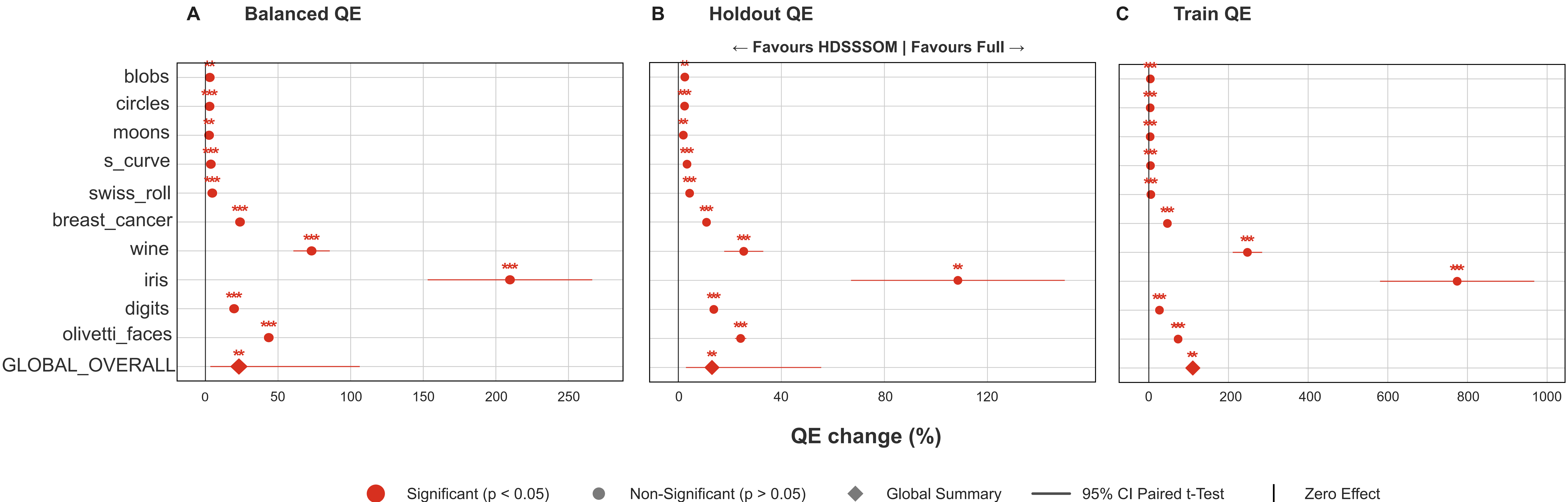
Figure 3: Full versus HDSSSOM on Pilot Dataset
