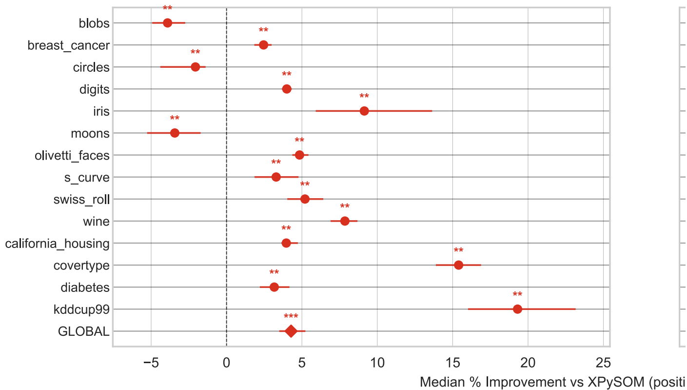
A Balanced QE
