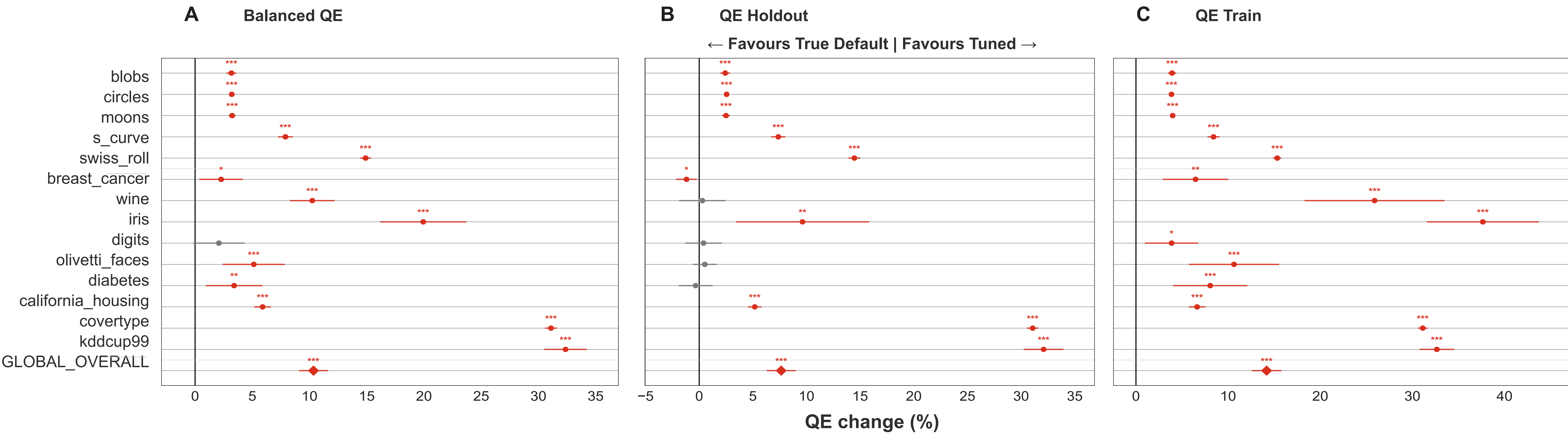
Supplementary Figure S8: Tuned vs True Default Across QE Metrics (Hexagonal)
