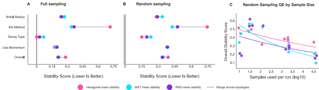
Figure 11: Hyperparameter Stability
