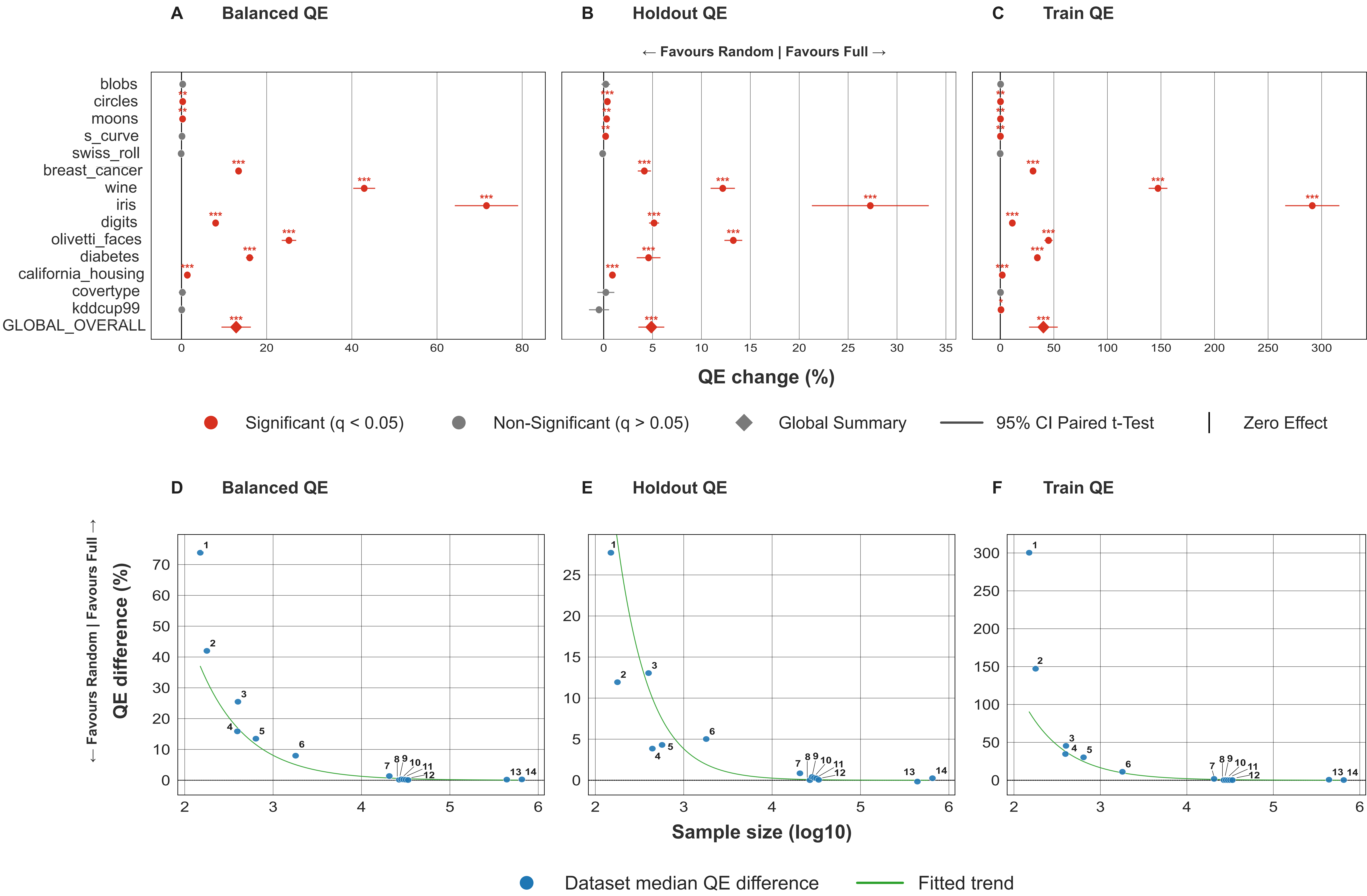
Figure 4: Full vs Random Outcomes and Dataset-Size Regression (Hexagonal)
