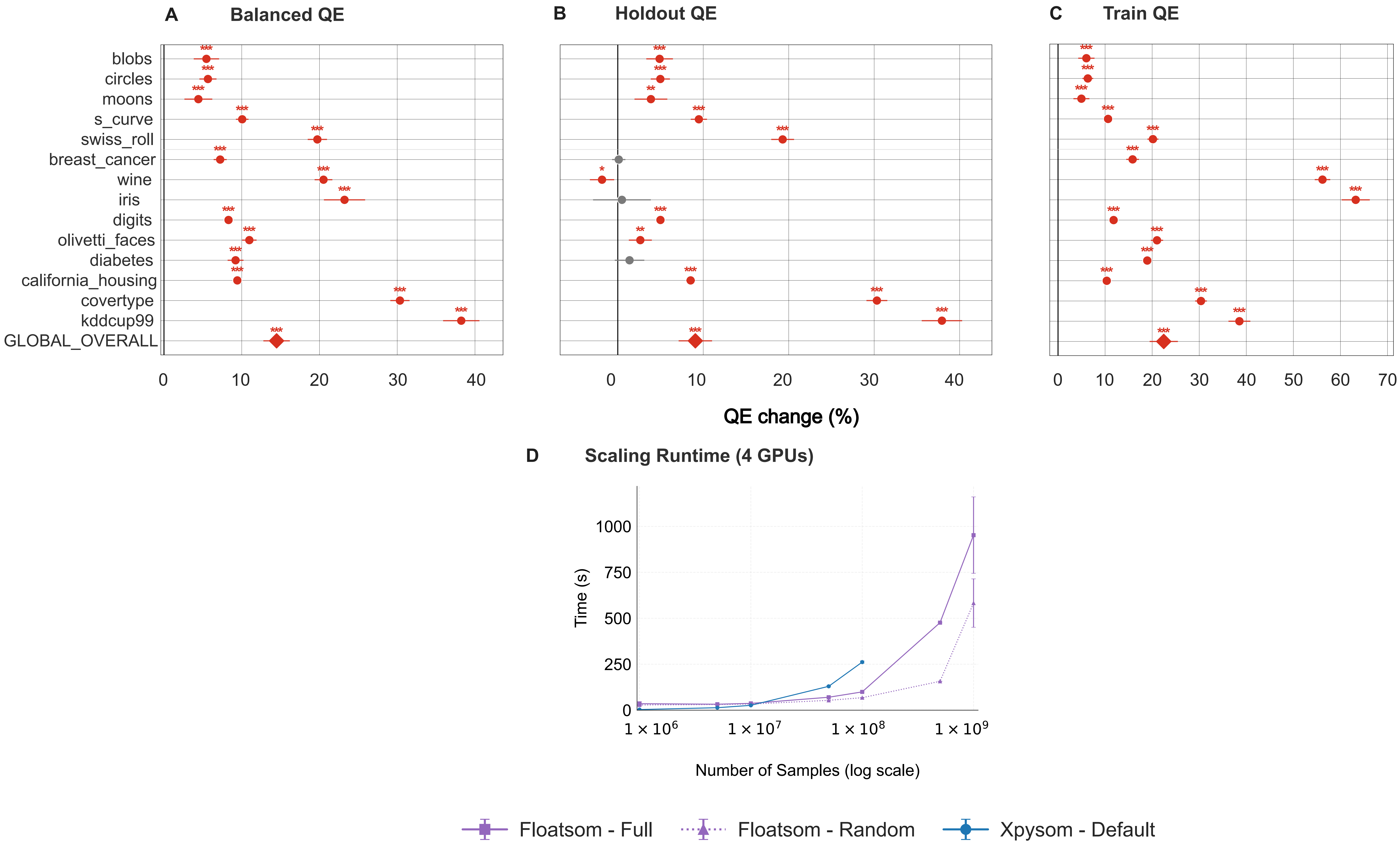
Figure 13: XPySOM (Default) v FloatSOM RNG
