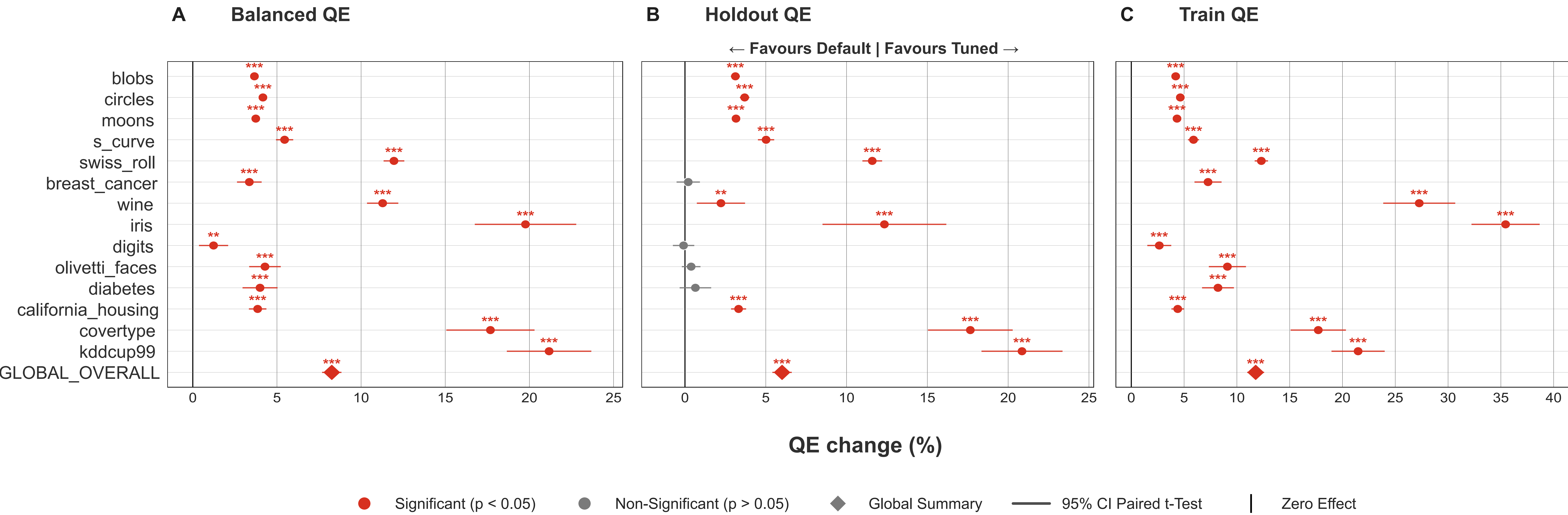
Figure 8: Tuned vs Default Across QE Metrics
