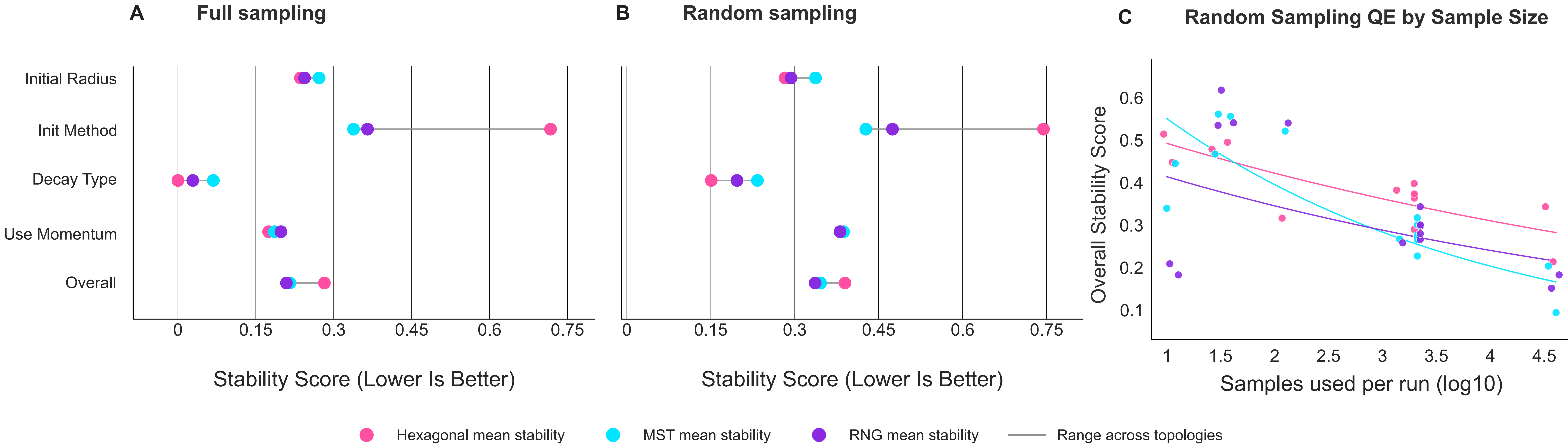
Figure 9: Hyperparameter Stability
