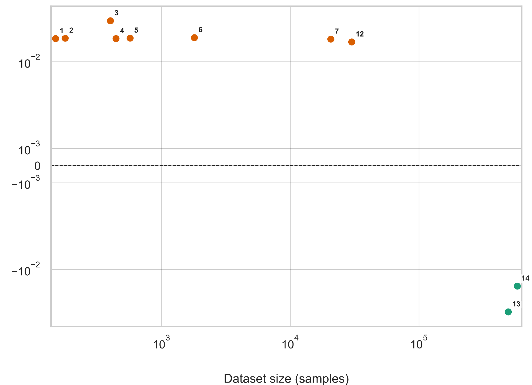
D Runtime Delta vs Dataset Size
