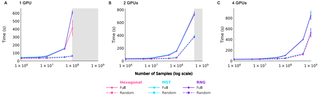
Figure 10: Sampling Runtime
