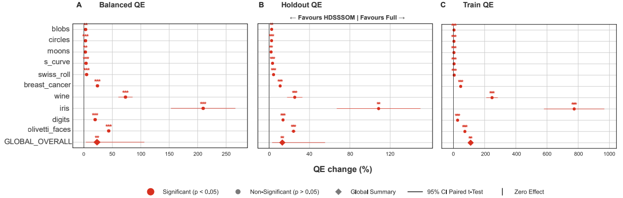
Figure 3: Full versus HDSSOM on Pilot Dataset
