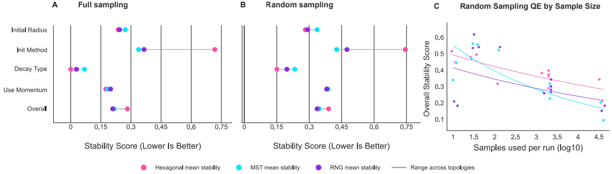
Figure 9: Hyperparameter Stability
