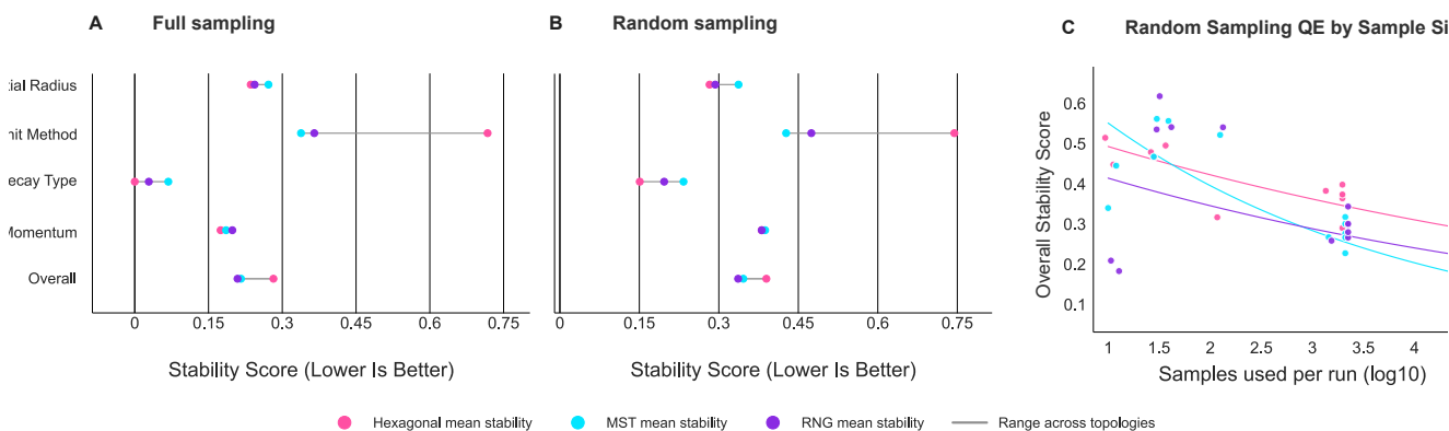
Figure 8. Hyperparameter stability by sampling mode. A: selected-parameter stability under full sampling for hexagonal, MST, and RNG topologies (lower stability score is better). B: selected-parameter stability under random sampling for the same topologies. C: dataset-size stability regression under random sampling, using the selected-parameter stability score against sample size (log10) across the included topology families.
