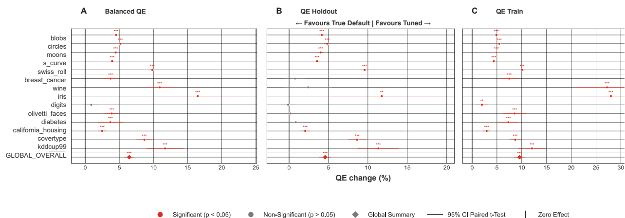
lementary Figure S10: Tuned vs True Default Across QE Metrics (MST)
