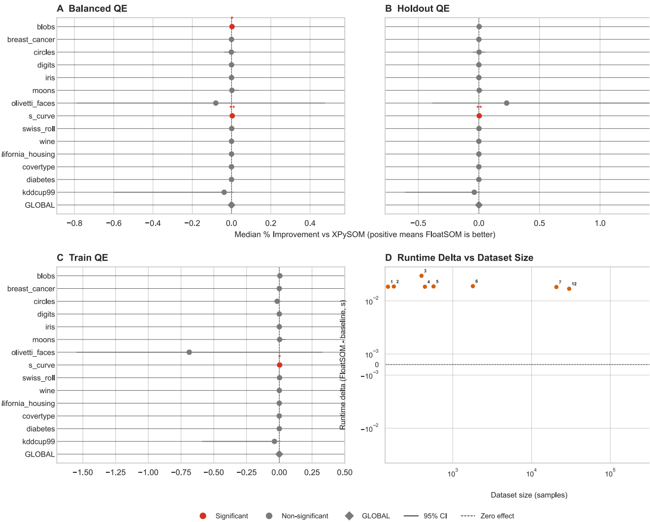
lementary Figure S3: FloatSOM vs XPySOM Calibration (Default Settings, Hexagonal)
