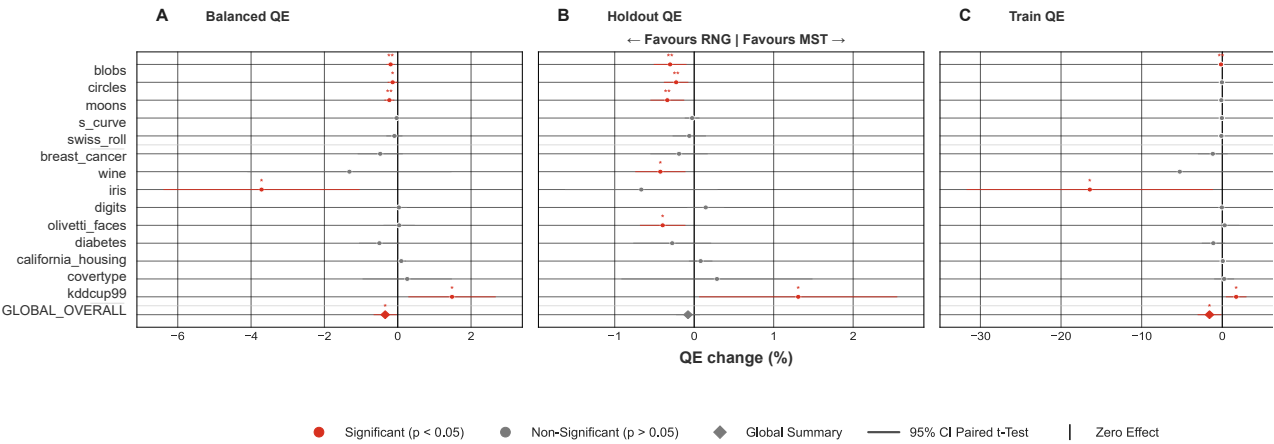
lementary Figure S5: MST vs RNG Across QE Metrics
