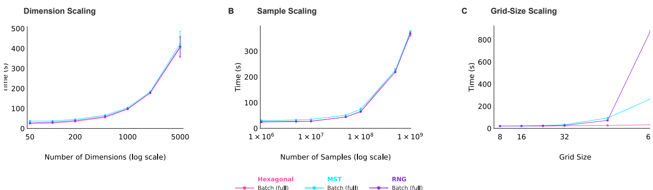
Figure 10: Topology Runtime Comparison (8 GPUs, Full Batch)
