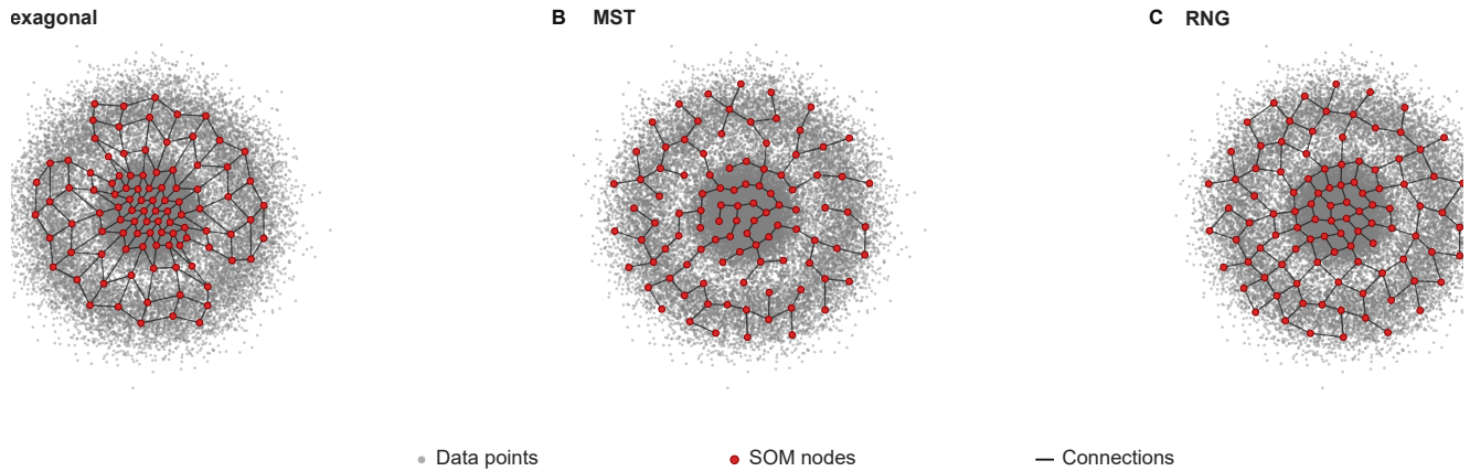
Figure 4. Representative figure for XPySOM default run Hexagonal, MST, and RNG neighborhood node and connection overlays on a 30,000 datapoint synthetic sklearn circles dataset.
