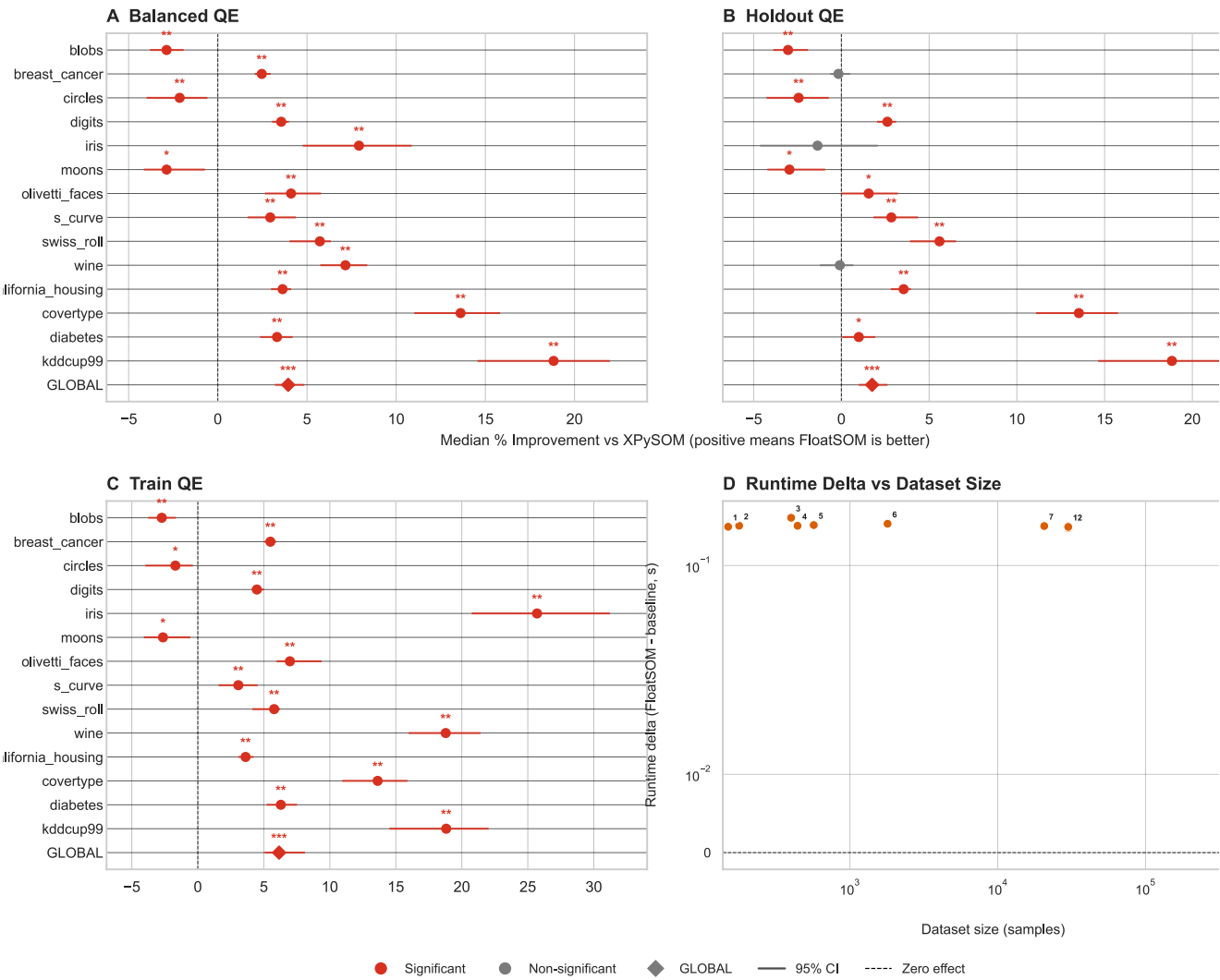
Supplementary Figure S2: FloatSOM vs XPySOM Calibration (Default Settings, RNG)
