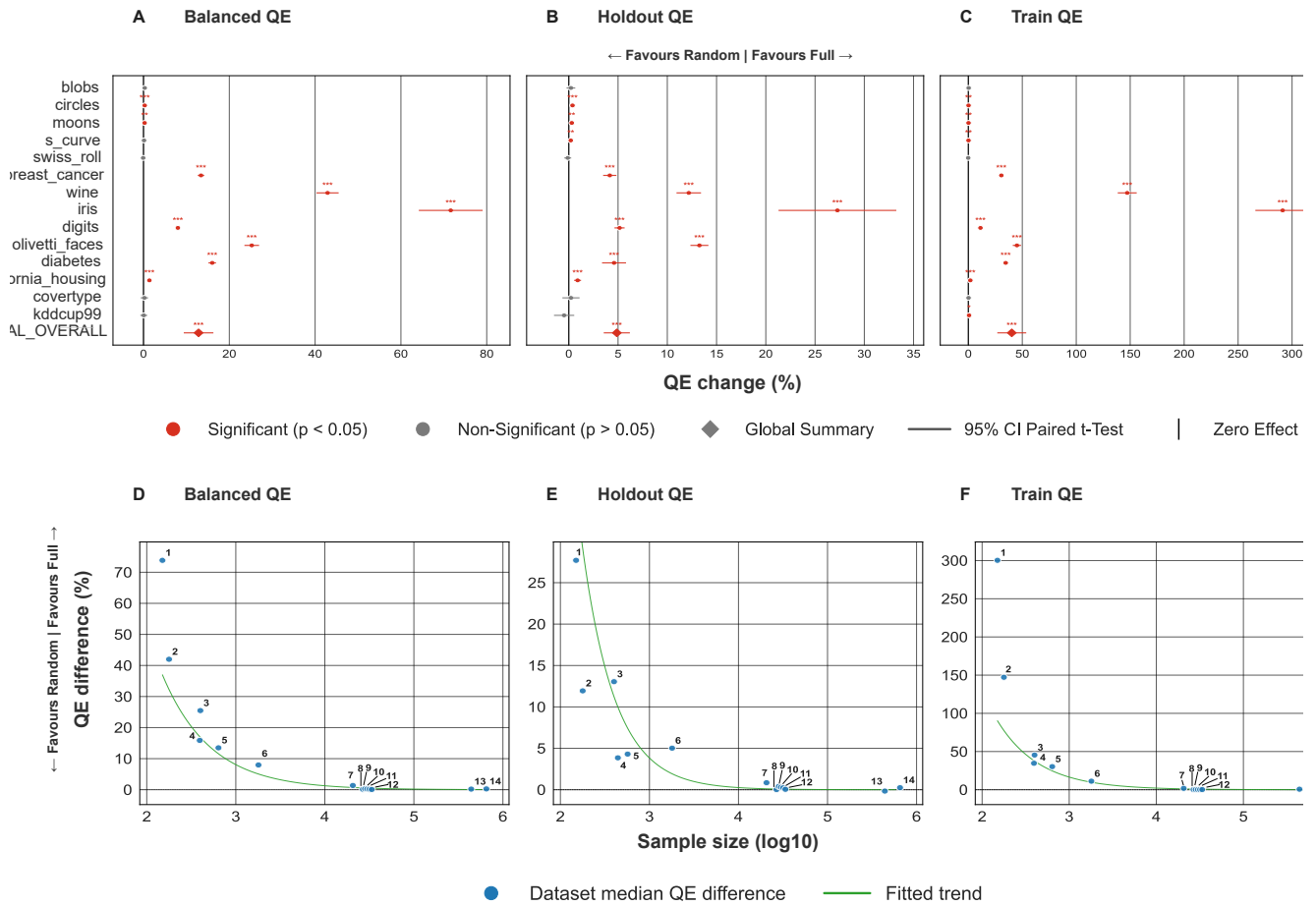
Figure 2: Full vs Random Outcomes and Dataset-Size Regression (Hexagonal / Full Batch)
