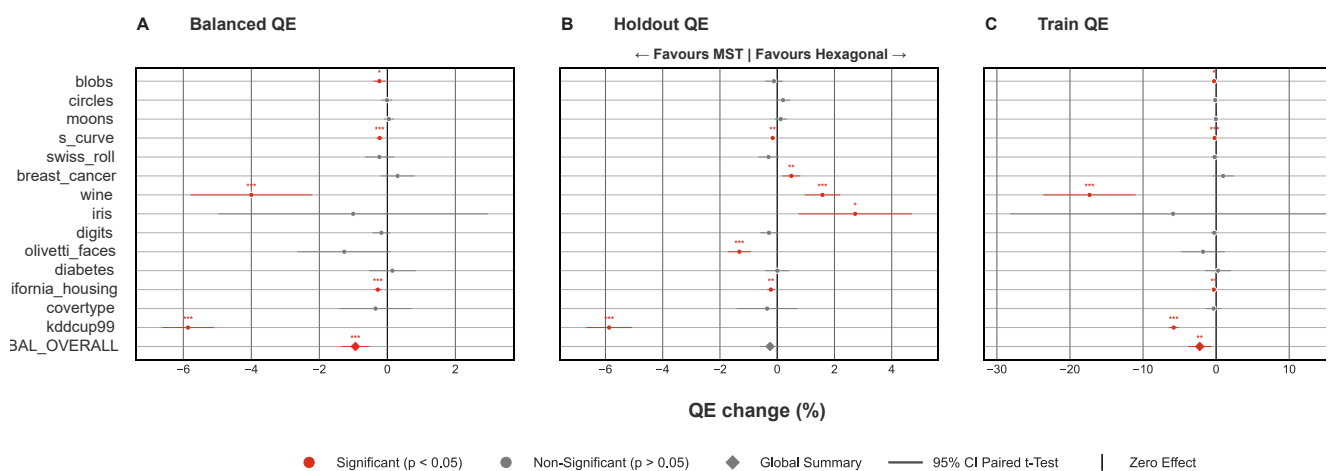
Figure 5. Hexagonal versus MST topology on QE endpoints under full sampling only. Panels A-C report paired full-sampling-only QE effects for QE_B , QE_H , and QE_T across the available full-sampling datasets. Forest whiskers denote 95% paired t-test confidence intervals around the mean paired effect.
