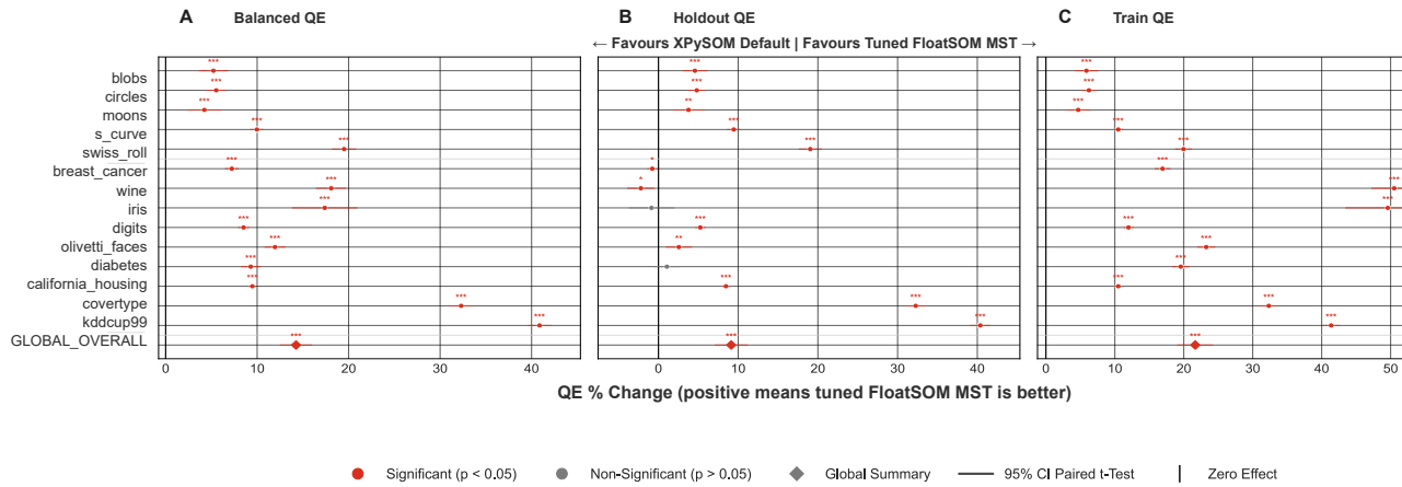
lementary Figure S14: XPySOM (Default) v FloatSOM MST
