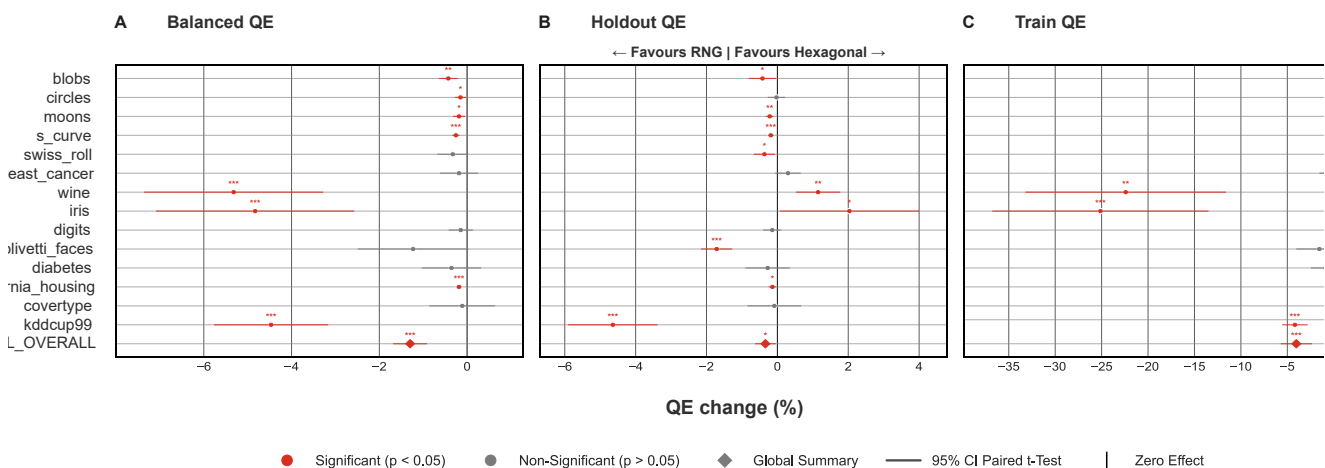
Figure 6. Hexagonal versus RNG topology on QE endpoints under full sampling only. Panels A-C report paired full-sampling-only QE effects for QE_B , QE_H , and QE_T across the available full-sampling datasets. Forest whiskers denote 95% paired t-test confidence intervals around the mean paired effect.
