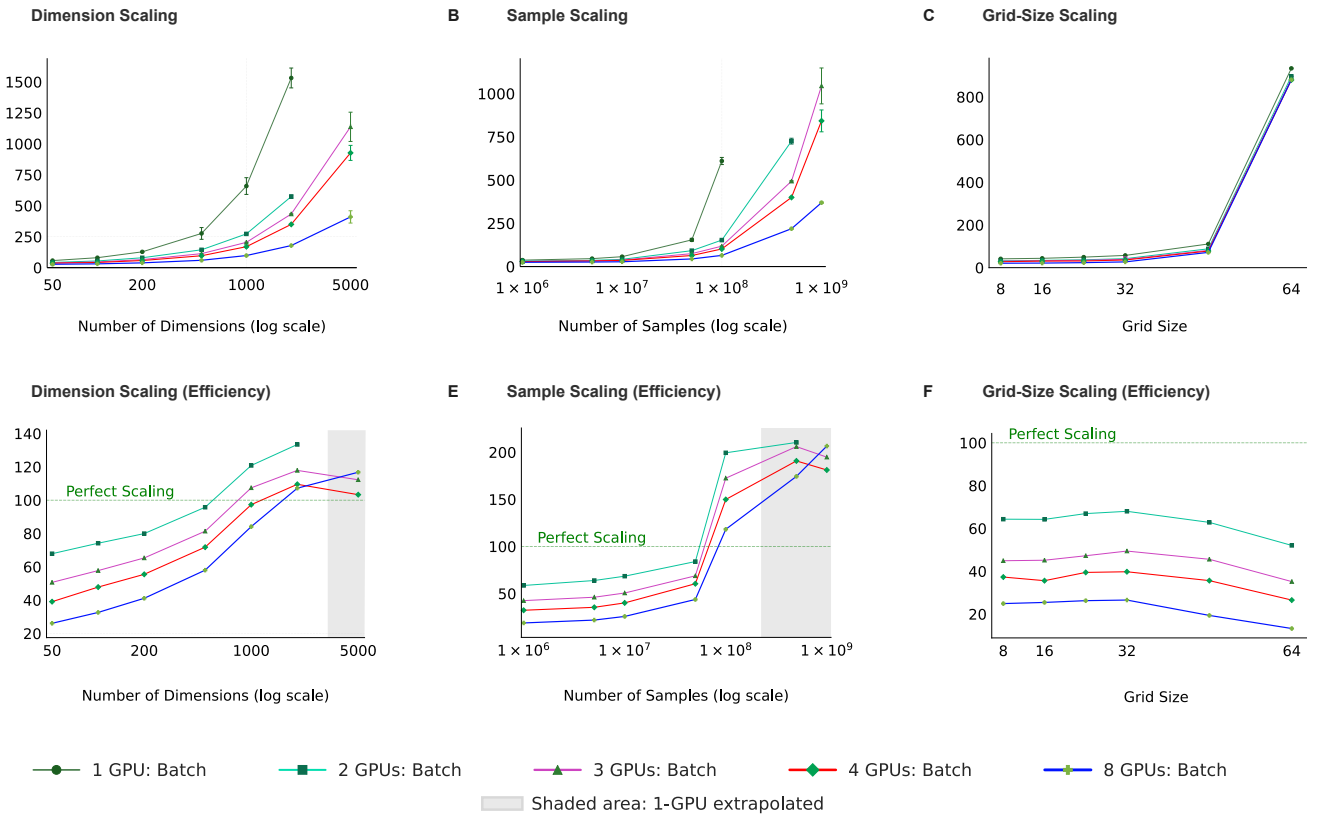
Figure 9: Multi-GPU Full-Batch Scaling (RNG)
