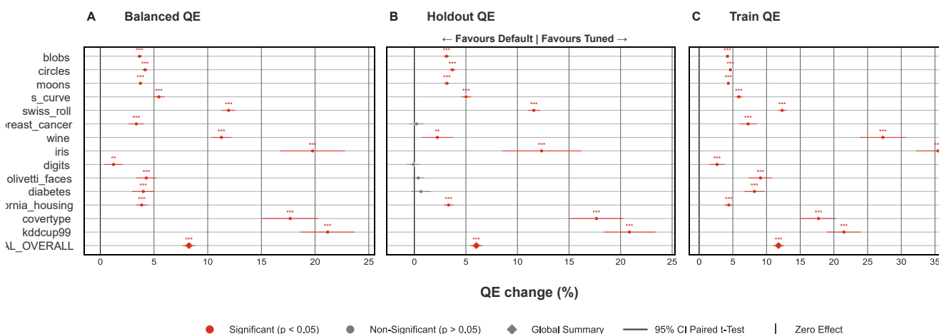
Figure 7. Tuned-configuration-versus-untuned-reference QE comparison across QE_B , QE_H , and QE_T , pooled across all topology runs under the matched pairing keys. Positive values indicate the tuned configuration outperforms the untuned reference; the global overall row pools all matched tuned-configuration/untuned-reference pairs across datasets. Forest whiskers denote 95% paired t-test confidence intervals around the mean paired effect.
