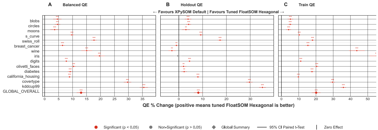
Supplementary Figure S12. Deployment comparison of default hexagonal XPySOM versus tuned FloatSOM hexagonal. Panels A-C report paired QE effects for QE_B , QE_H , and QE_T under the matched dataset/seed comparison keys. Positive values indicate tuned FloatSOM hexagonal outperforms default hexagonal XPySOM. Forest whiskers denote 95% paired t-test confidence intervals around the mean paired effect. Per-dataset and GLOBAL_OVERALL panel summaries are listed in Supplementary Table S8.
