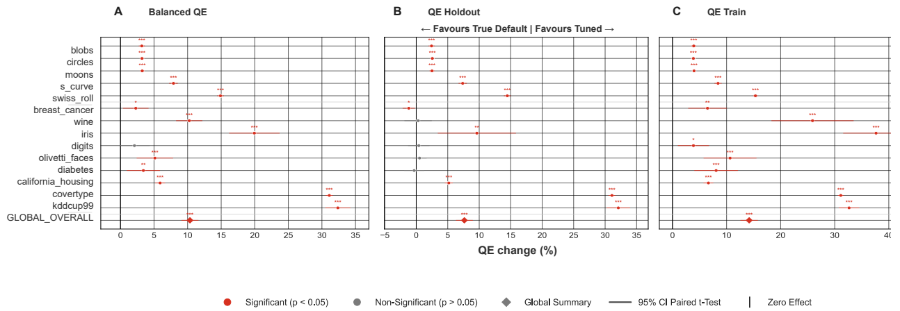
Supplementary Figure S8. Tuned-configuration-versus-untuned-reference QE comparison for the hexagonal topology only, across QE_B , QE_H , and QE_T under the matched pairing keys. Positive values indicate the tuned configuration outperforms the untuned reference. Forest whiskers denote 95% paired t-test confidence intervals around the mean paired effect.
