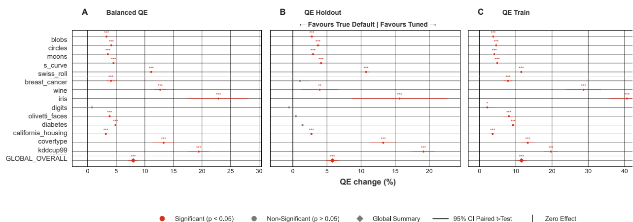
lementary Figure S11: Tuned vs True Default Across QE Metrics (RNG)
