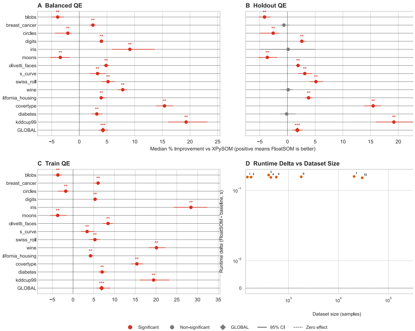
Supplementary Figure S1: FloatSOM vs XPySOM Calibration (Default Settings, MST)
