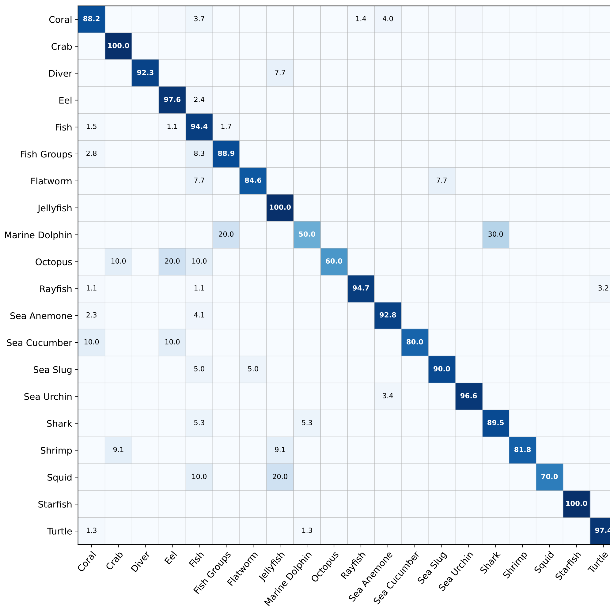
Predicted class
