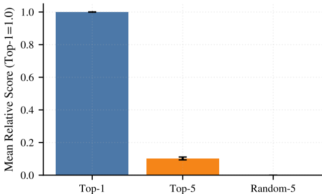
F2 Top-k vs Random Model: allenai/OLMo-7B-0724-hf
