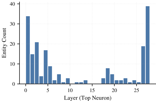
Entity-Neuron Layer Distribution (PopQA, n=200)
