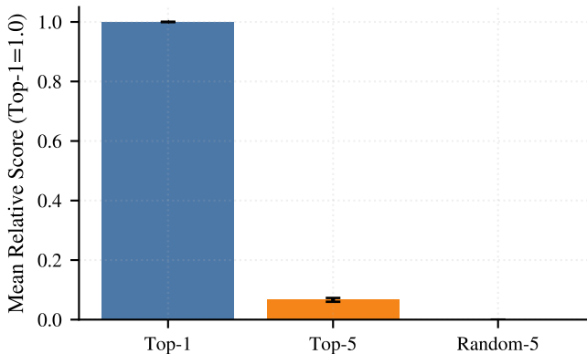
F2 Top-k vs Random Model: Qwen/Qwen2.5-7B-Instruct
