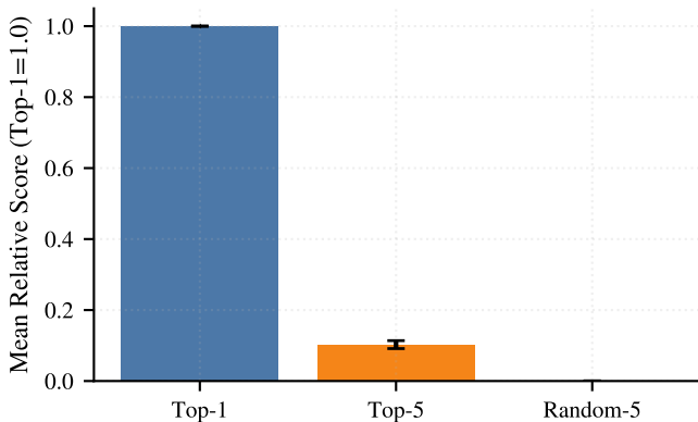
F2 Top-k vs Random Model: openlm-research/open_llama_7b
