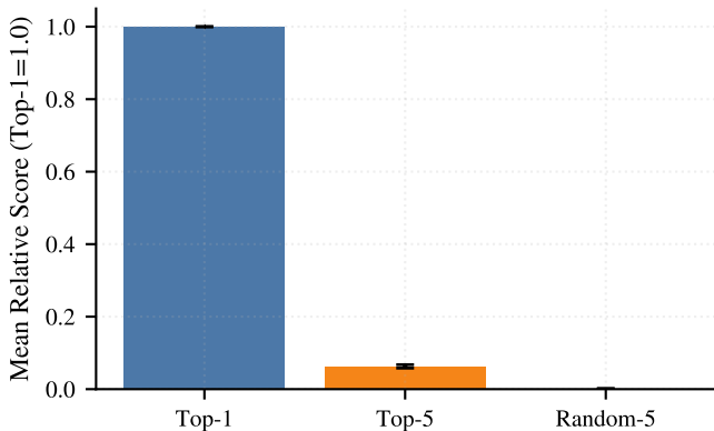
F2 Top-k vs Random Model: meta-llama/Llama-3.1-8B-Instruct
