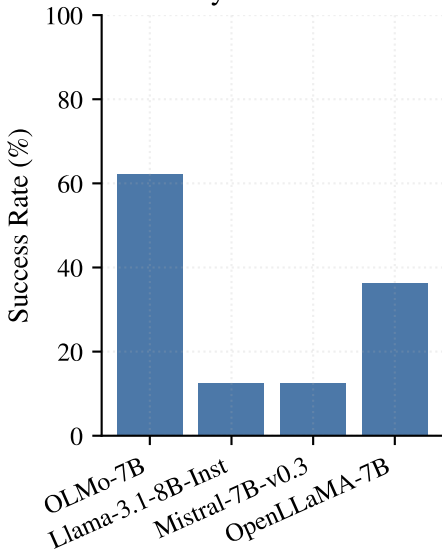
Entity-level success
