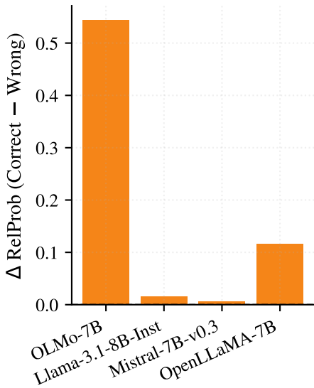
Causal separation
