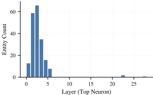
Top-Neuron Layer Distribution
