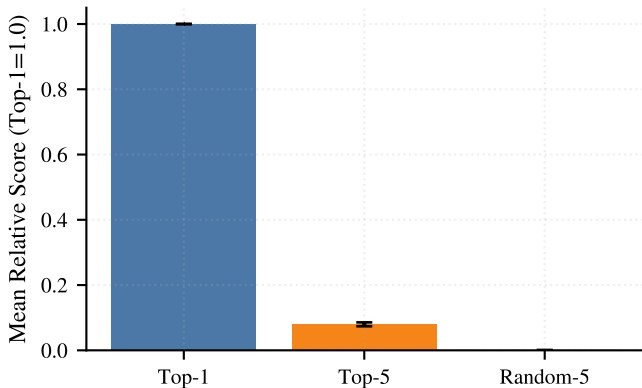
F2 Top-k vs Random Model: Qwen/Qwen3-8B
