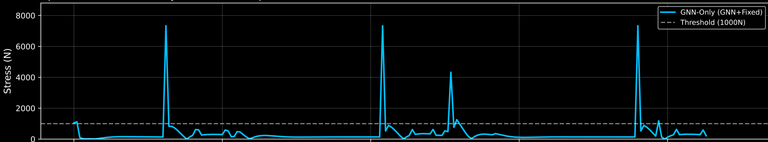
Episode Trace: No-Curriculum (peak=7419.0N)
