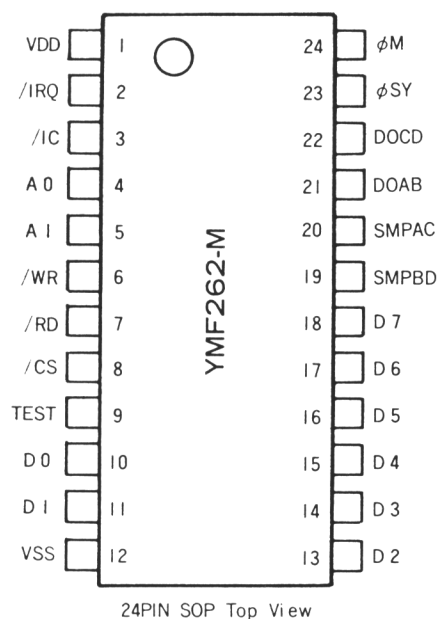
24PIN SOP Top View
