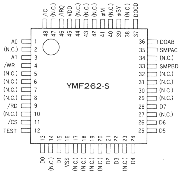
48pin SQFP top view
