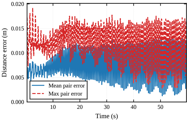
S1 Hover: formation keeping
