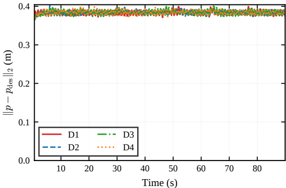
S2 Circle: tracking error
