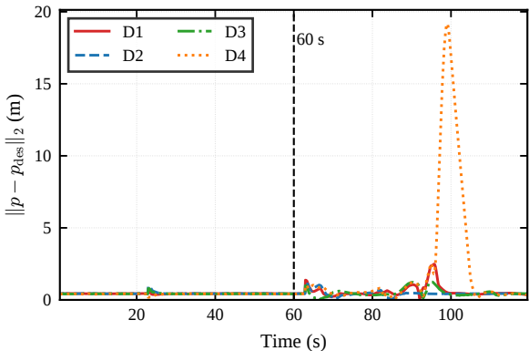
S3 Reconfiguration: tracking error
