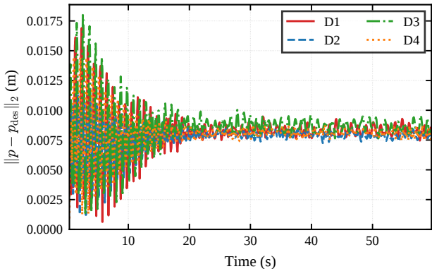
S1 Hover: tracking error
