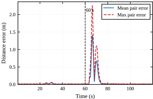
S3 Reconfiguration: formation keeping
