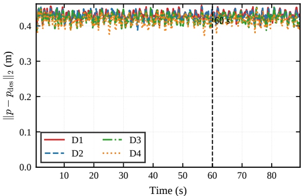
S4 Wind Disturbance: tracking error
