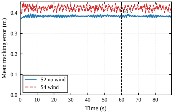
Wind disturbance effect
