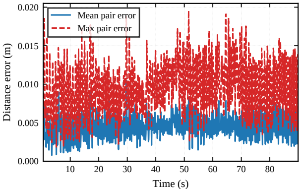
S2 Circle: formation keeping
