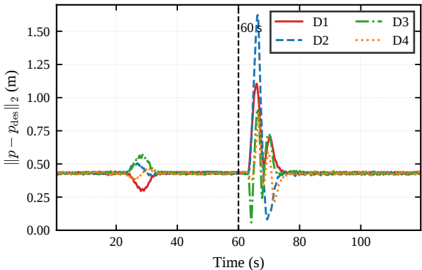
S3 Reconfiguration: tracking error
