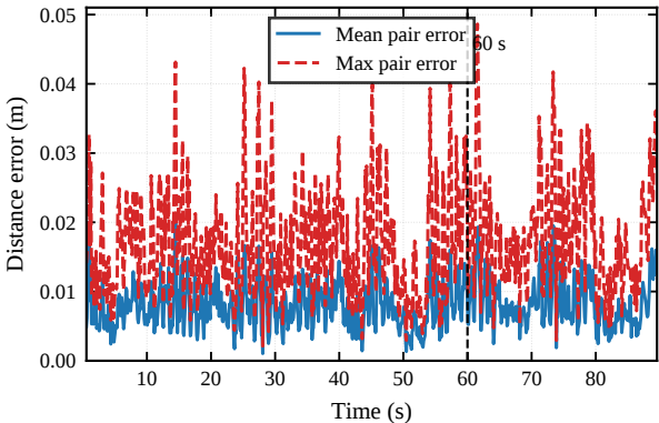
S4 Wind Disturbance: formation keeping
