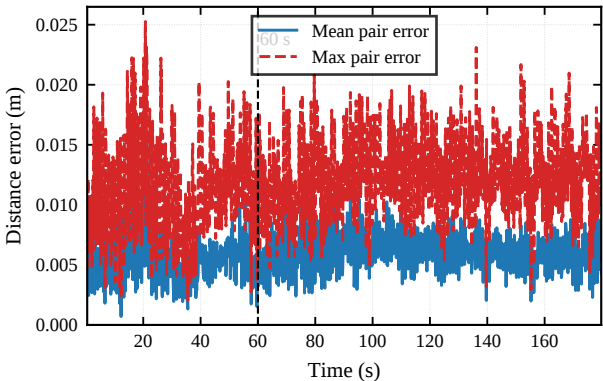
S5 Long-Duration: formation keeping
