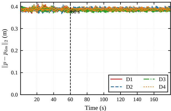
S5 Long-Duration: tracking error
