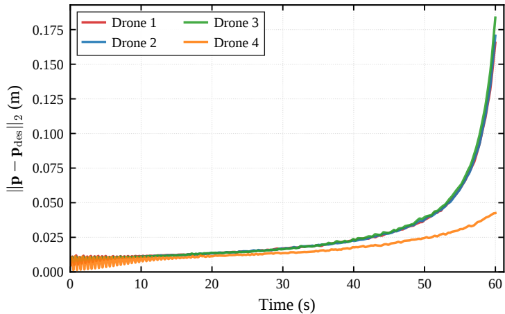
S1: Static Hover: 3D Tracking Error
