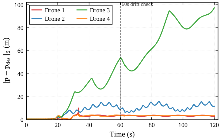
S3: Formation Reconfig.: 3D Tracking Error
