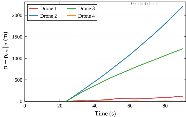
S4: Wind Disturbance: 3D Tracking Error
