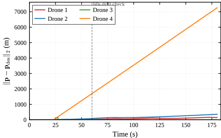
S5: Long-Duration Flight: 3D Tracking Error
