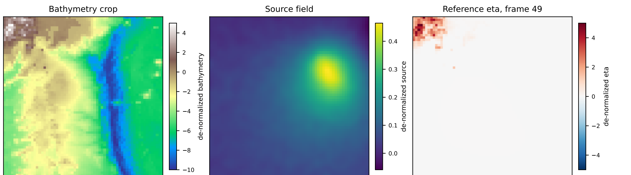
Coastline wet-dry
