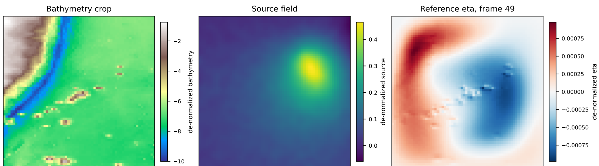
Offshore morphology
