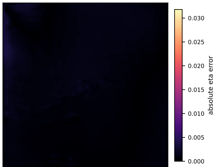
Window-FNO-5 |error| rel-L2=0.038
