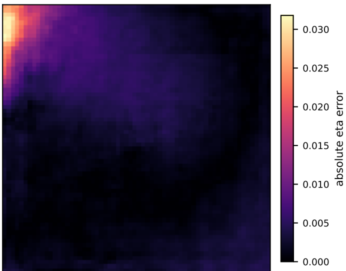
Direct-FNO |error| rel-L2=0.291
