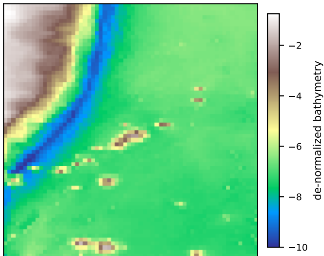
Bathymetry crop
