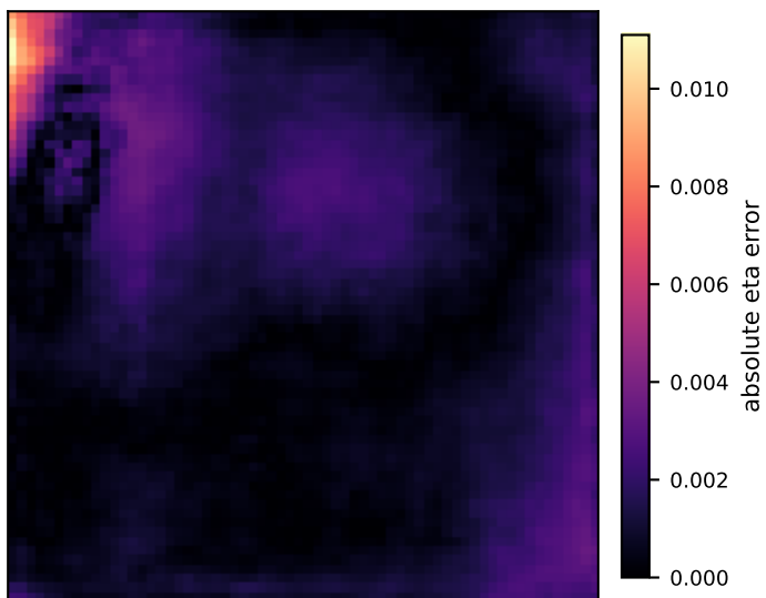
Direct-FNO |error| rel-L2=0.212
