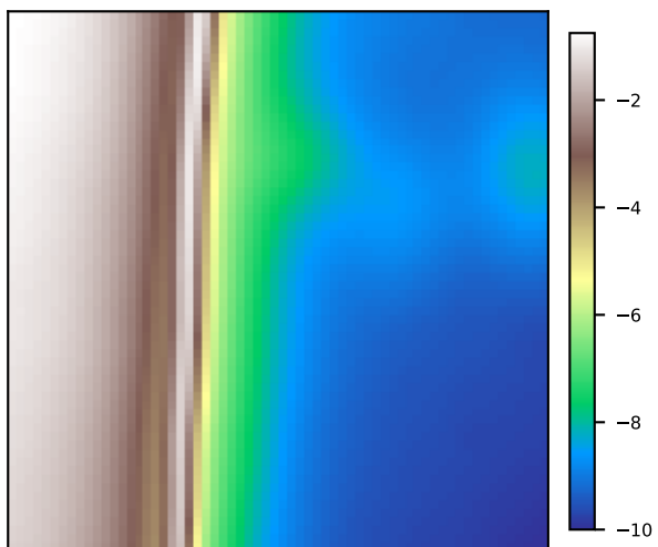
Bathymetry
