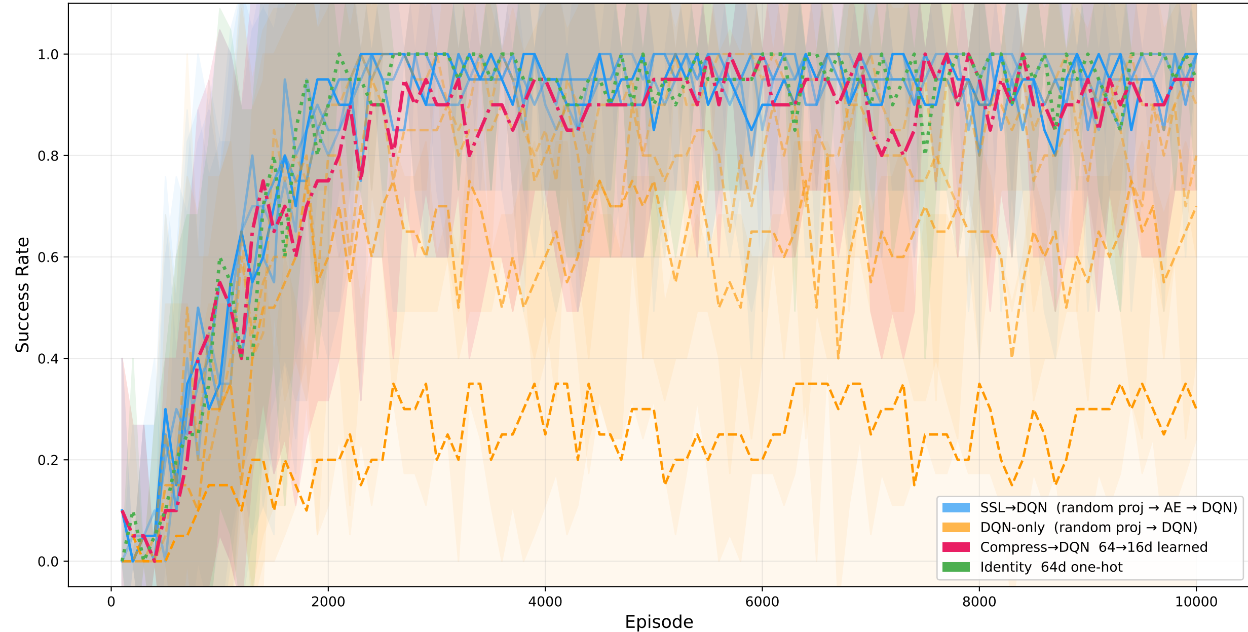
DQN Learning Curves: All Pipelines
