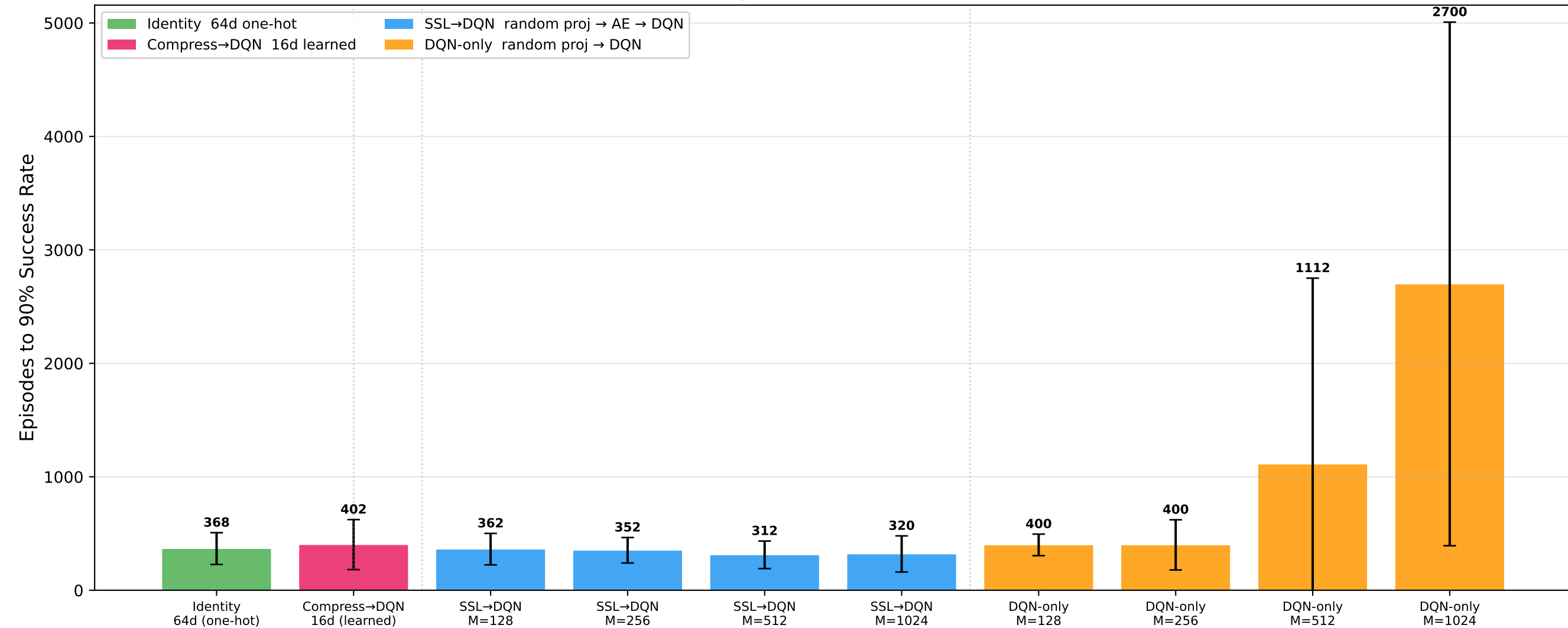
Sample Efficiency: Episodes to 90% Success Rate
