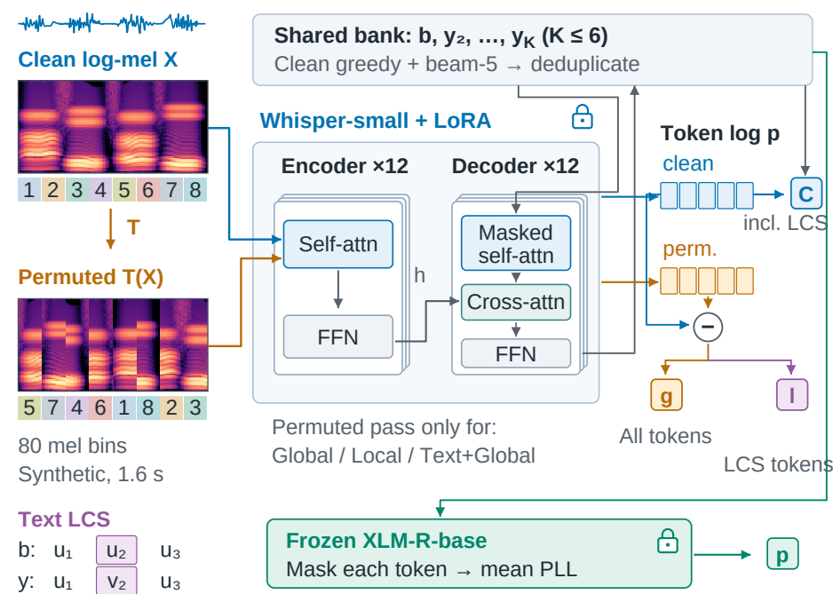
(a) Frozen models and shared candidate evidence
