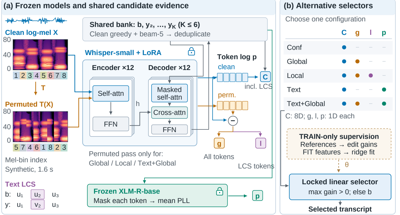
Fig. 1. Frozen reranking architecture. (a) Shared Whisper generation/scoring; only Global, Local and Text+Global use the permuted pass. XLM-R supplies PLL. Synthetic mel blocks and text LCS illustrate permutation and disagreement, not acoustic alignment. (b) Alternative fits: C includes local clean confidence; g/l/p denote global/local contrasts and PLL. Dashed links carry TRAIN coefficients; locks mark frozen models.
