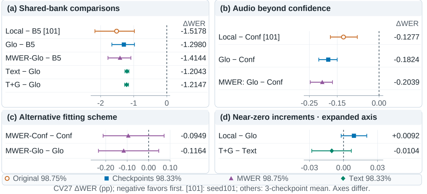
Fig. 2. Paired CV27 WER differences. [101] marks seed101-only rows (Original, 98.75%); others average three checkpoints (Checkpoints/Text, 98.33%, rounded; MWER, 98.75%). Intervals condition on fixed fits. Glo=Global, T+G=Text+Global. MWER: Glo–Conf compares MWER fits. Axes differ; (d) expands zero.
